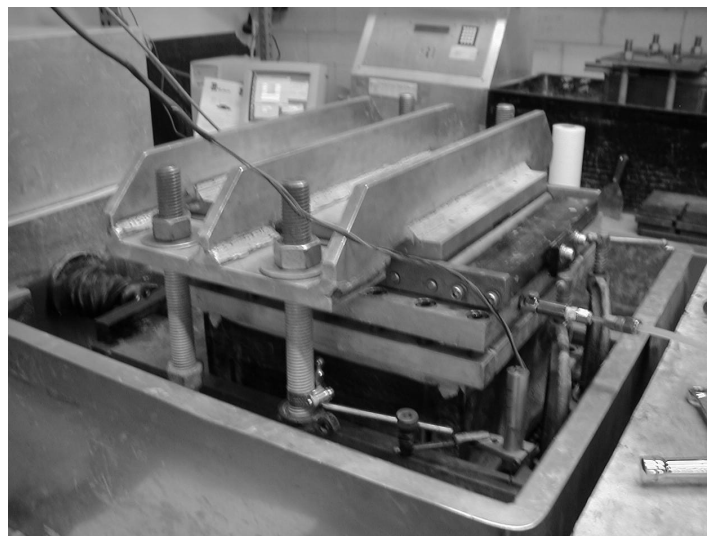
Figure 6: Large Shear Box
